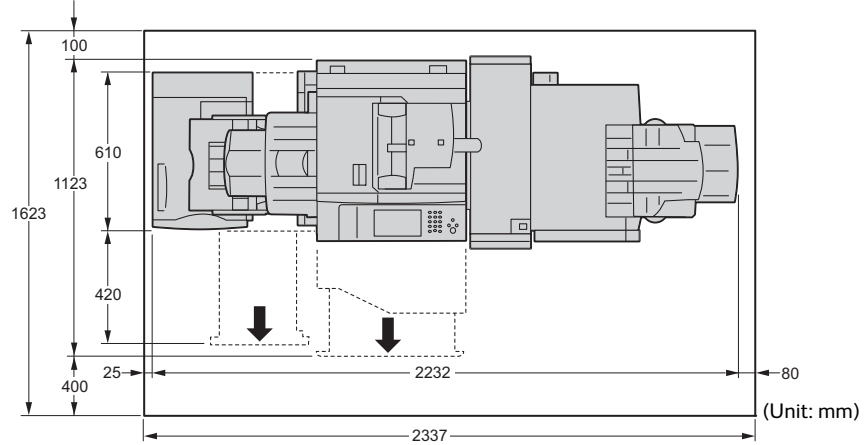
With C3 Finisher with Booklet Maker (optional), Folder Unit CD1 (optional), HCF B1 (optional), and Side Tray (optional)
